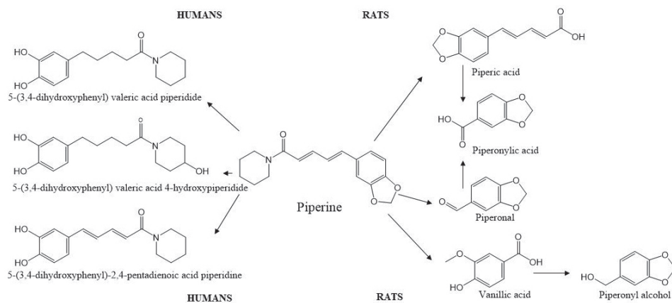
Fig. 5. Structure of piperine and metabolites identified in human and rat urine (12).
