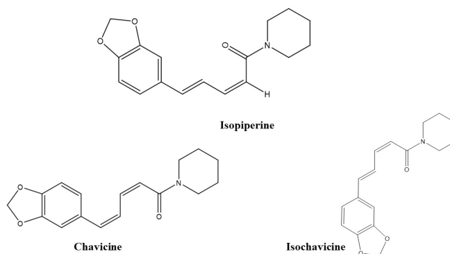
Fig. 2. Alkaloids obtained from black pepper ( P. nigrum L.): chavicine, isopiperine and isochavicine (7, 132).
