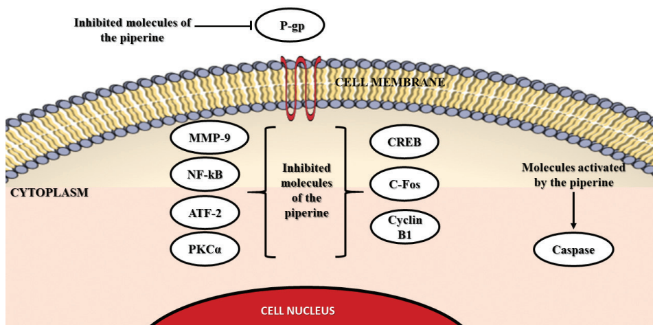
Fig. 7. The schematic diagram of the molecular machinery and possible targets for the antineoplastic properties of piperine. ATF-2 – activated transcription factor 2, CREB – cAMP response element-binding, MMP-9 – matrix metalloproteinase 9, NF-κB – nuclear factor κ-light-chain-enhancer of activated B cells, PKC – protein kinase C.
