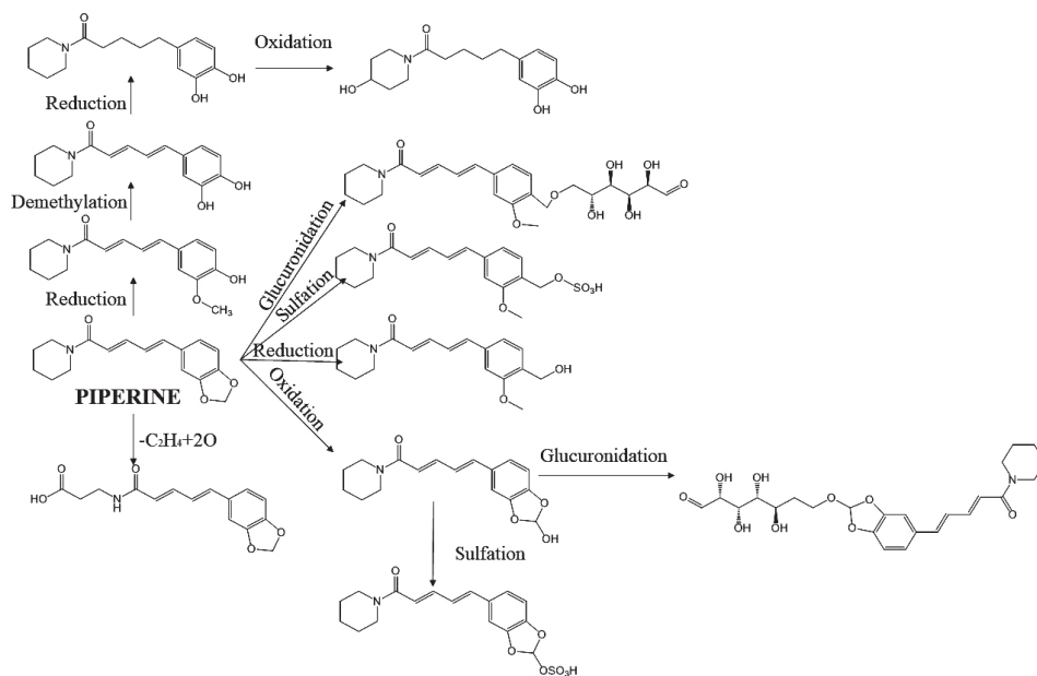
Fig. 6. Metabolic pathways of piperine identified after in vivo experiments with rats (133).
