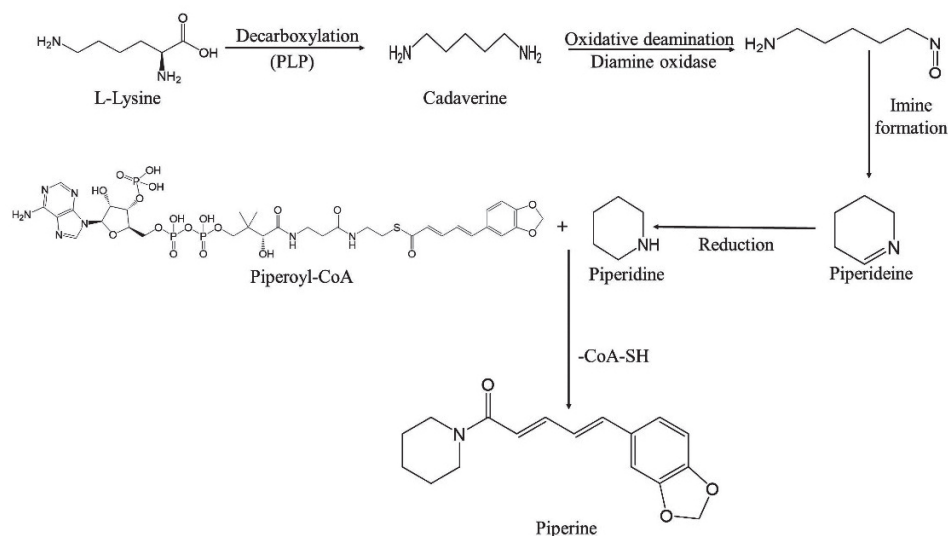
Fig. 3. Schematic representation of PIP biosynthesis from L-lysine (6).
