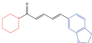
Fig. 1. Chemical structure of piperine. Three sub-units: butadiene chain (sub-unit in black), an amide function formed by piperidine and \alpha,\beta -unsaturated carbonyl (subunit in red), a piperonal nucleus (sub-unit in blue).
