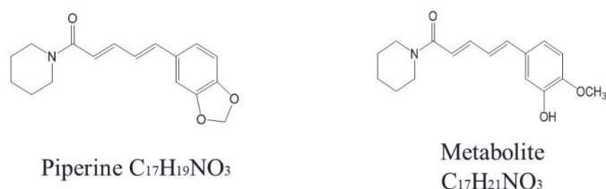
Fig. 4. Piperine and similar metabolites in human urine (4,5-dihydropiperine) (12).
