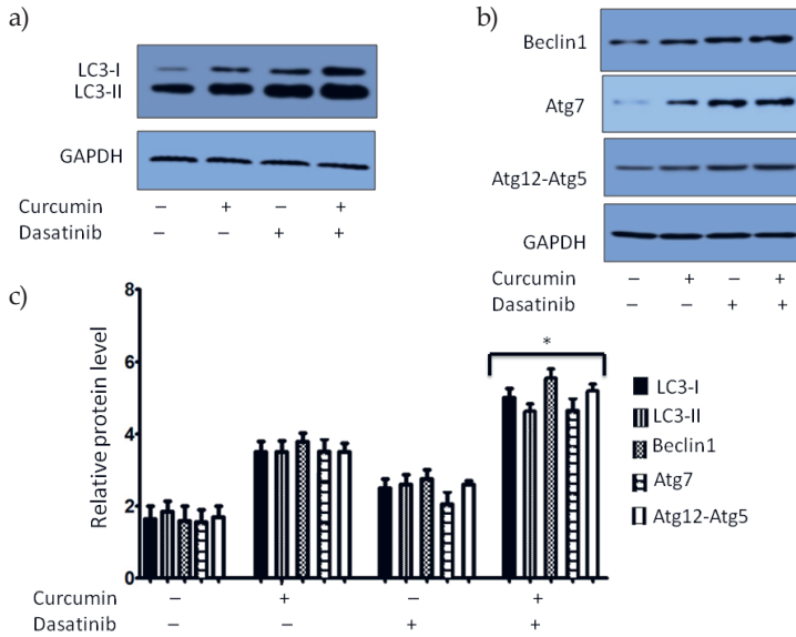
Fig. 3. a) and b) Expression analysis of autophagy-related marker proteins using immunoblotting (untreated cells – control; GAPDH – internal control), c) densitometry analysis.
